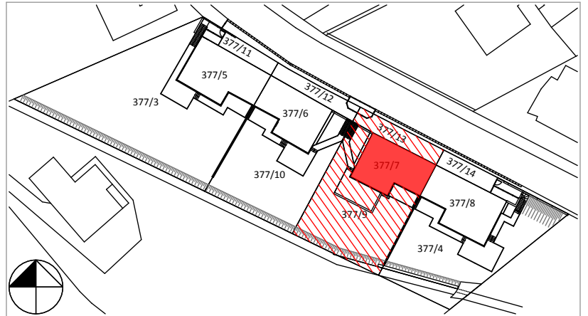
SITE PLAN - HOUSE POSITION
